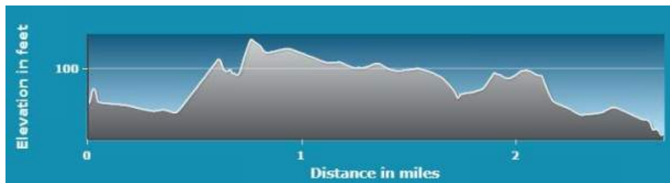
Figure 3-12 Seymour to Ansonia Conveyance Pipeline Profile
