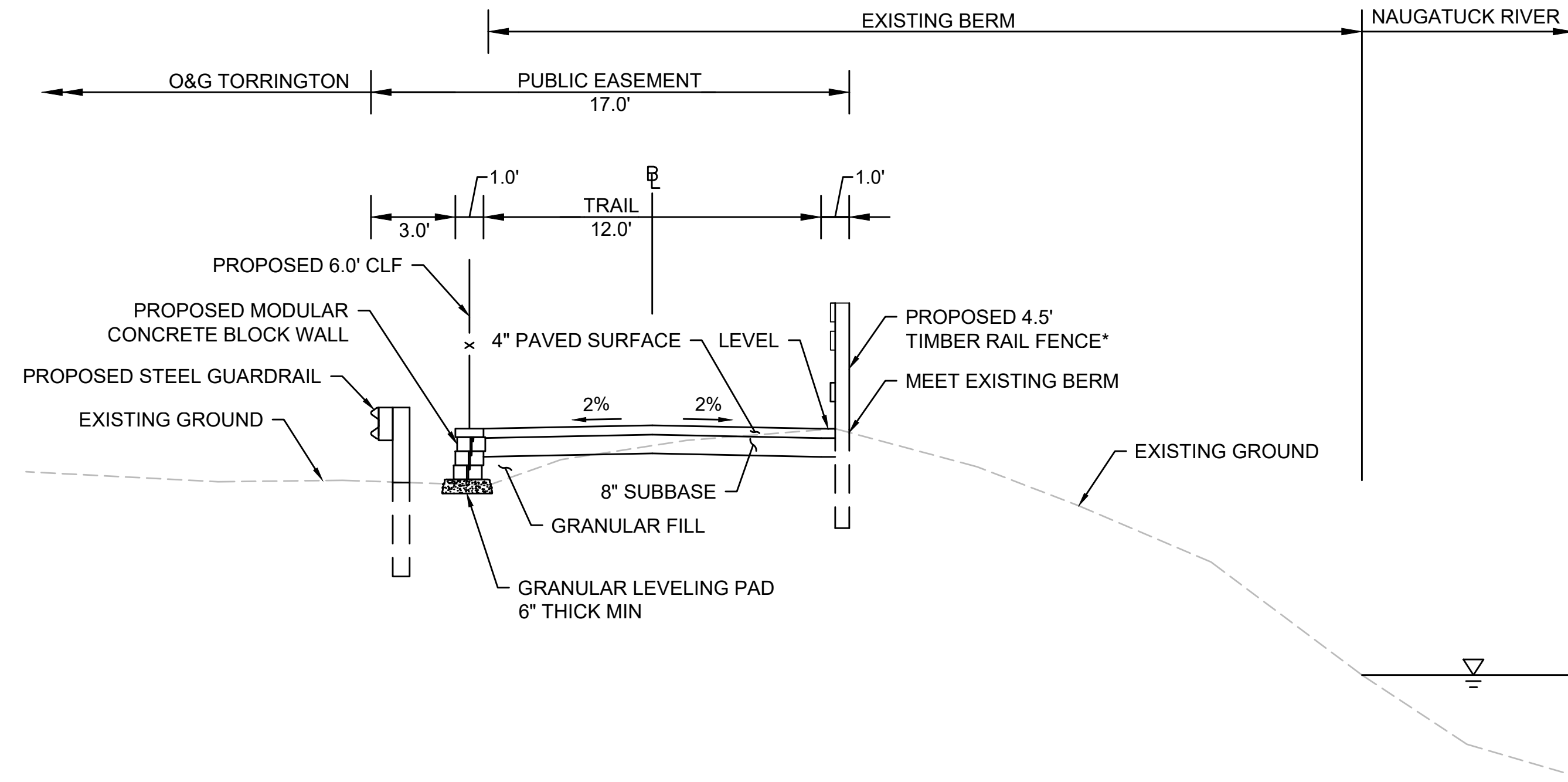
OFF-ROAD TRAIL ALONG O&G TORRINGTON BERM SCALE: 1" = 4'
