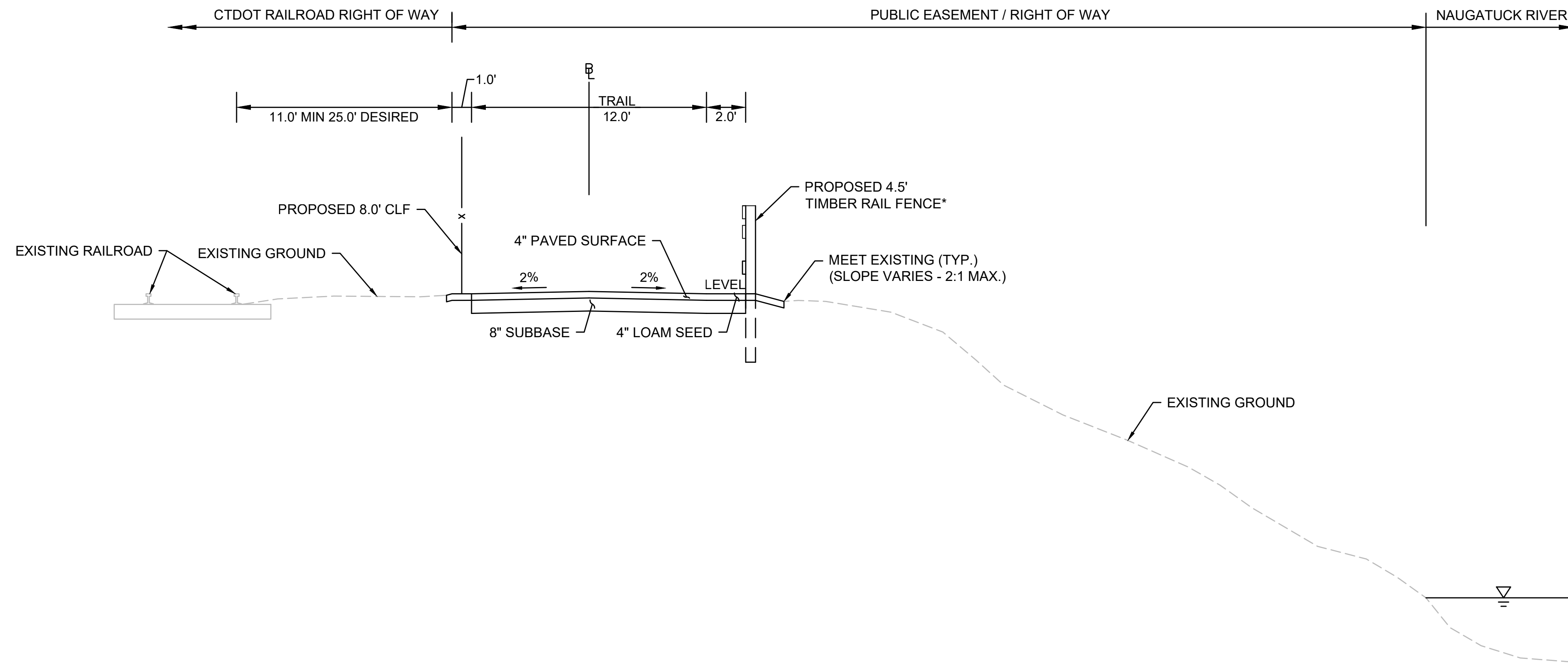
OFF-ROAD TRAIL NEAR / WITHIN RAILROAD RIGHT OF WAY SCALE: 1" = 4'
